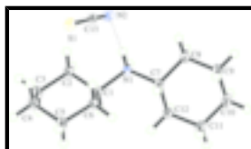
Fig. 1. Molecular structure of (I) showing atom-labelling scheme and displacement ellipsoids at the 30% probability level.
